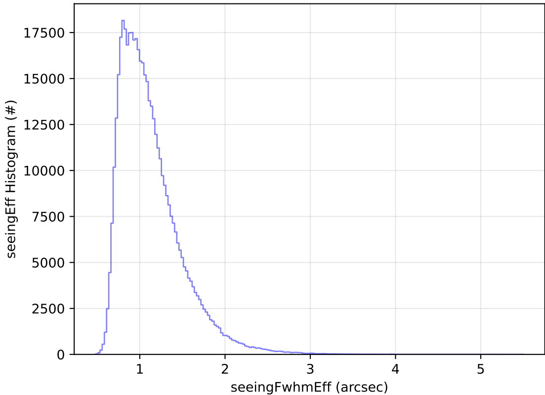
too_elab_r256_d2_griz_v3.4_10yrs All sky r band: seeingEff Histogram
