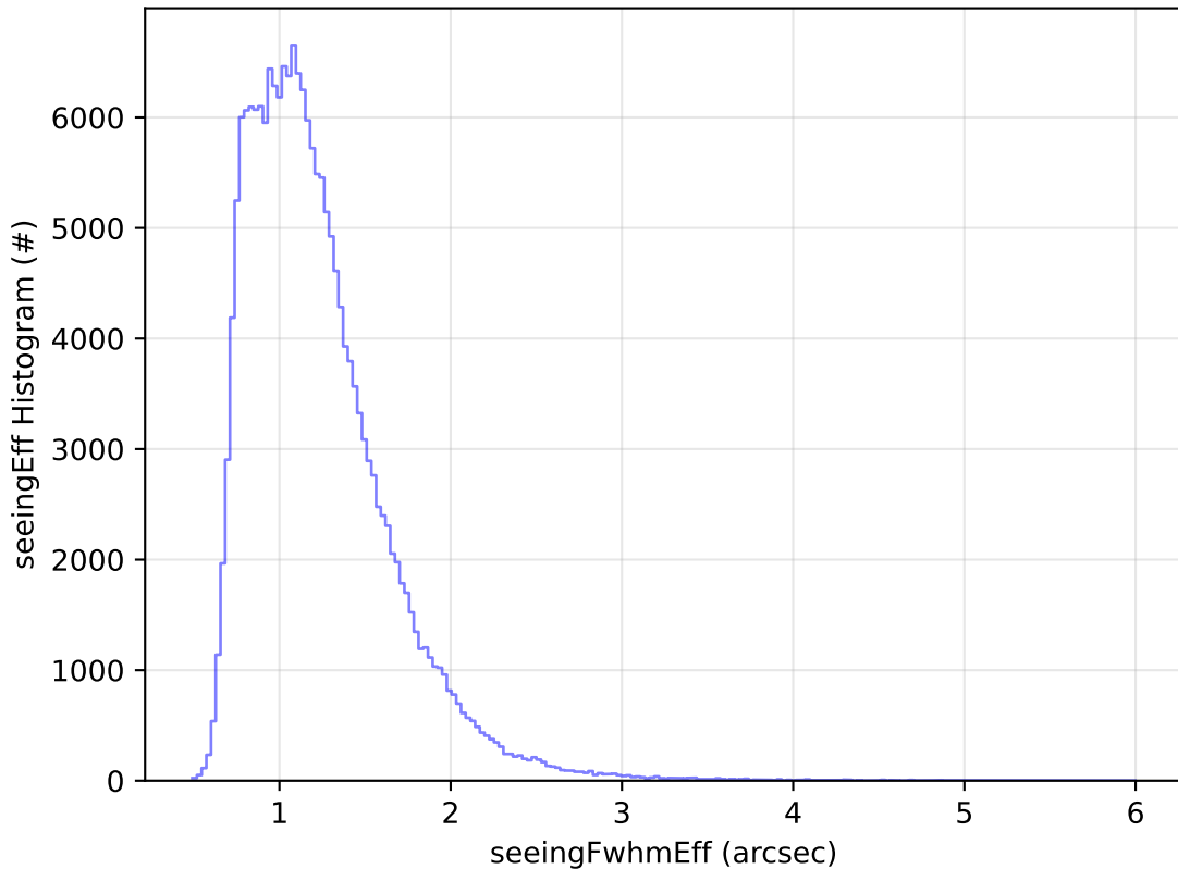
too_elab_r256_d2_griz_v3.4_10yrs All sky g band: seeingEff Histogram
