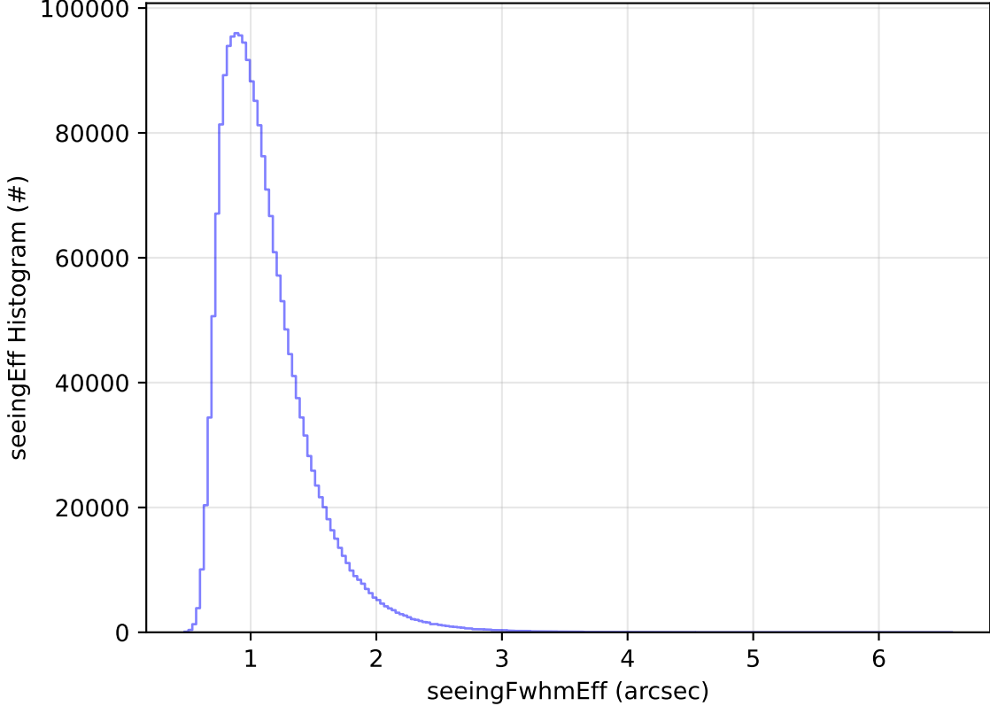
too_elab_r256_d2_griz_v3.4_10yrs All sky all bands: seeingEff Histogram
