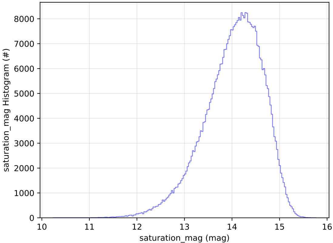
too_elab_r256_d2_griz_v3.4_10yrs WFD z band: saturation_mag Histogram
