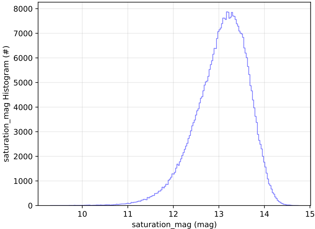
too_elab_r256_d2_griz_v3.4_10yrs WFD y band: saturation_mag Histogram
