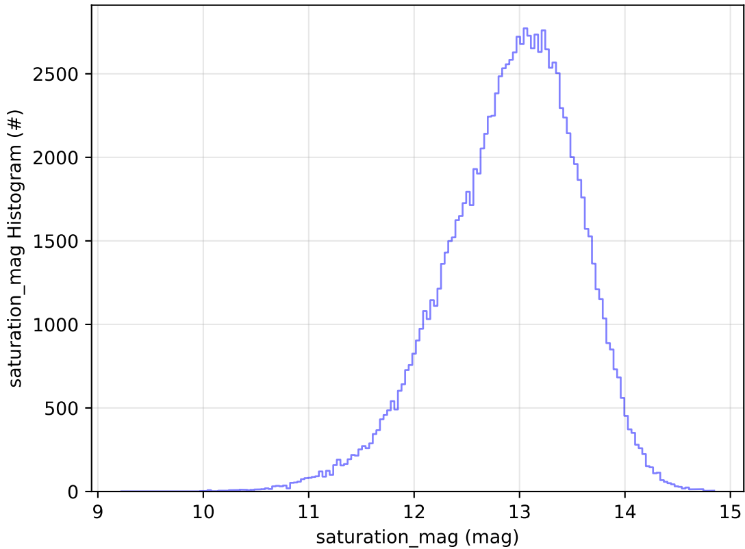
too_elab_r256_d2_griz_v3.4_10yrs WFD u band: saturation_mag Histogram
