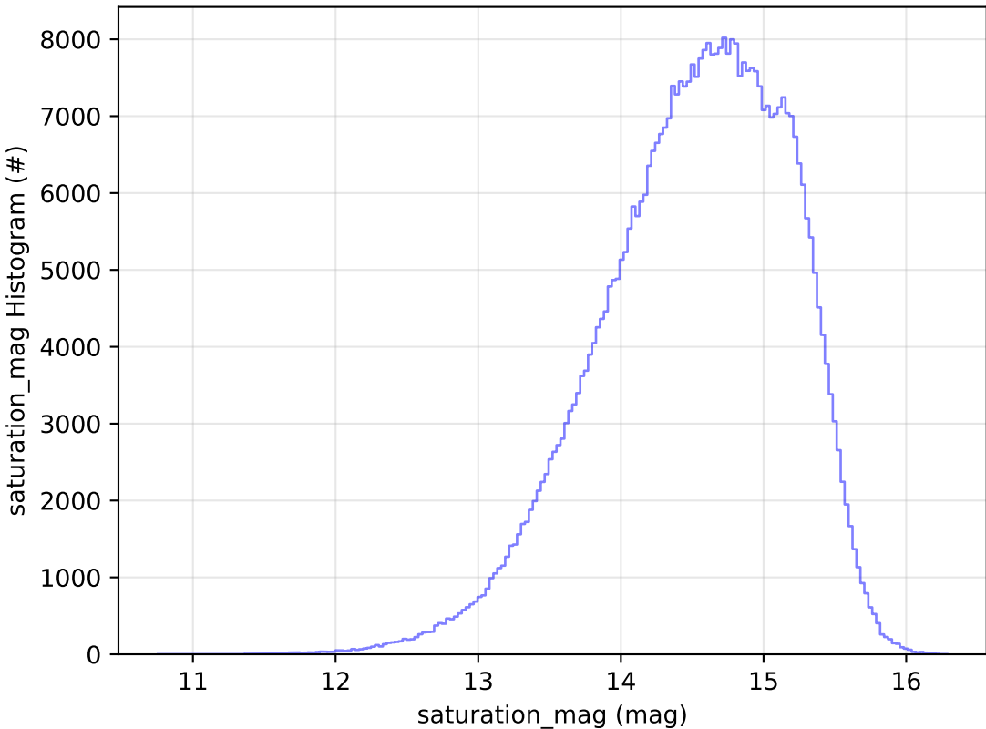
too_elab_r256_d2_griz_v3.4_10yrs WFD r band: saturation_mag Histogram
