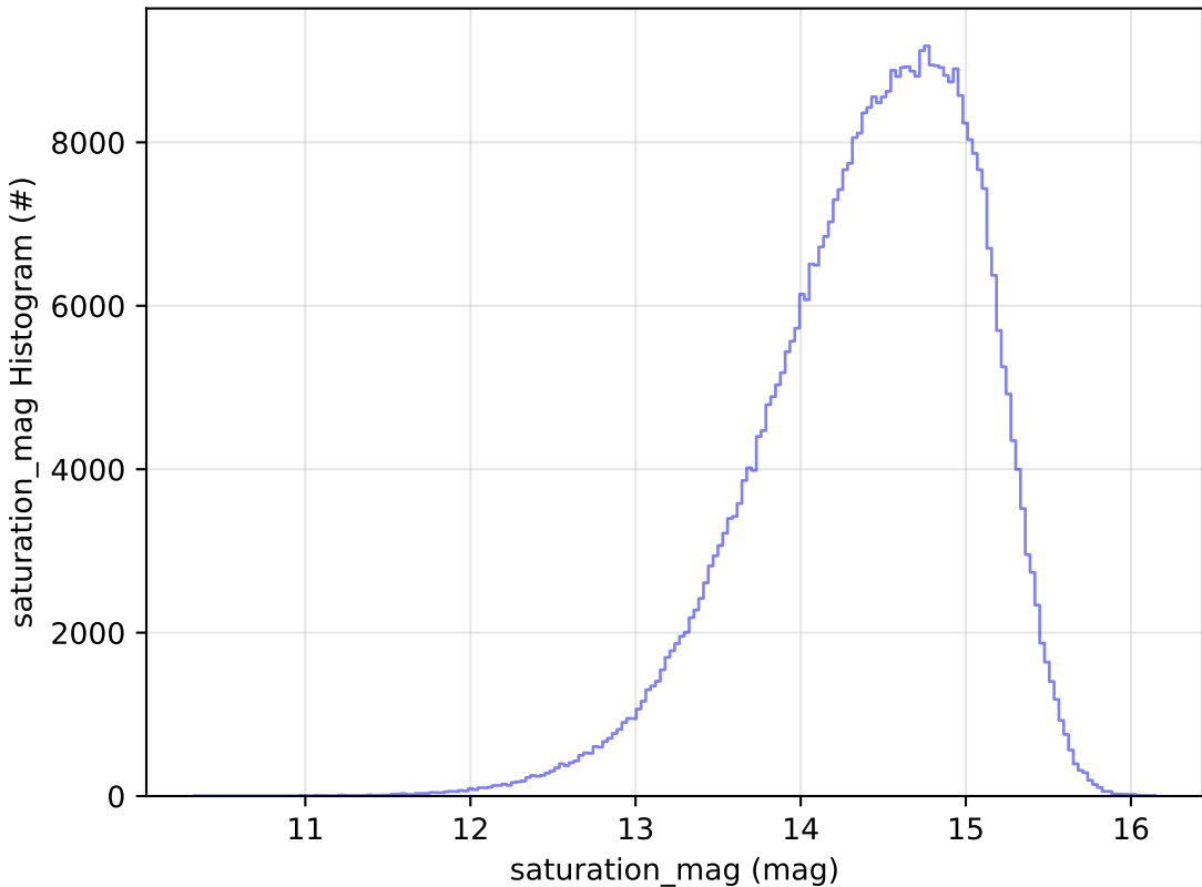
too_elab_r256_d2_griz_v3.4_10yrs WFD i band: saturation_mag Histogram
