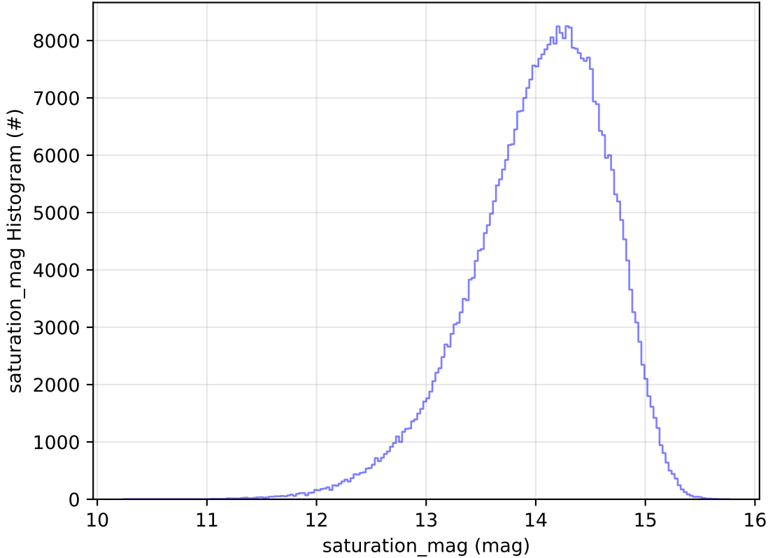
too_elab_r256_d2_griz_v3.4_10yrs All sky z band: saturation_mag Histogram
