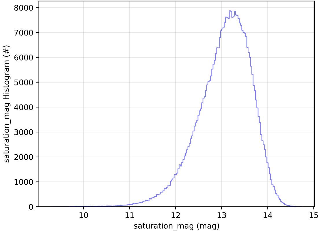
too_elab_r256_d2_griz_v3.4_10yrs All sky y band: saturation_mag Histogram
