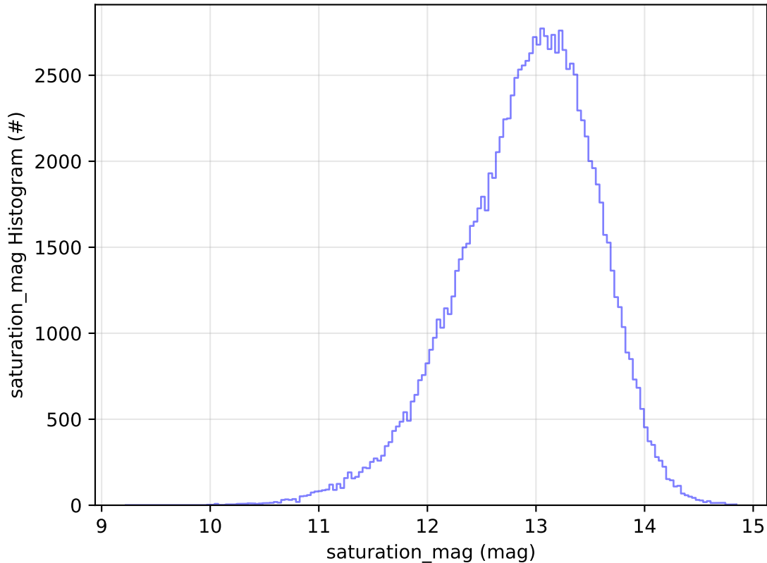
too_elab_r256_d2_griz_v3.4_10yrs All sky u band: saturation_mag Histogram
