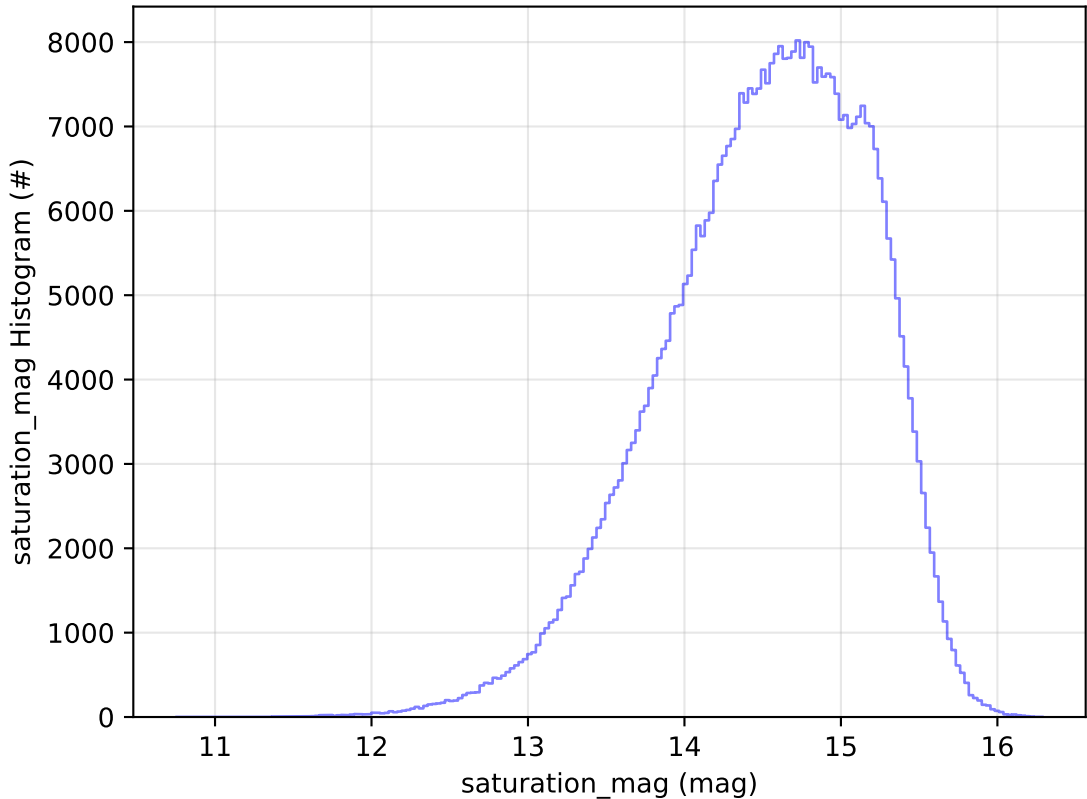
too_elab_r256_d2_griz_v3.4_10yrs All sky r band: saturation_mag Histogram
