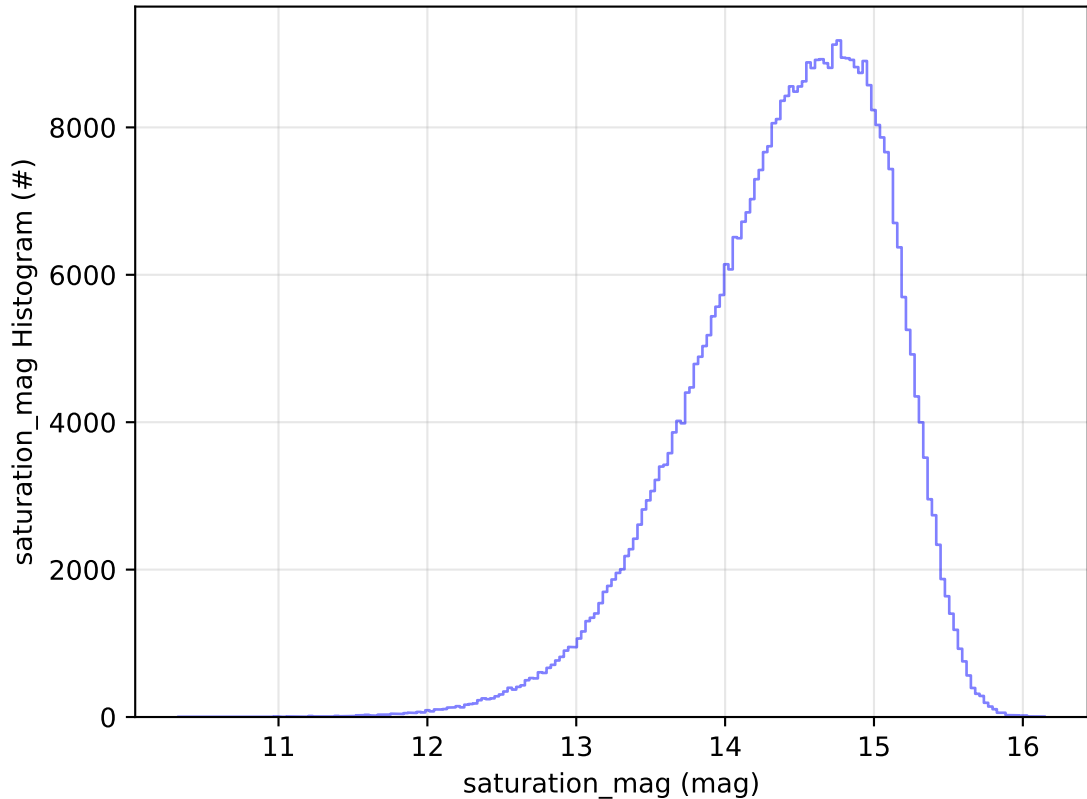
too_elab_r256_d2_griz_v3.4_10yrs All sky i band: saturation_mag Histogram
