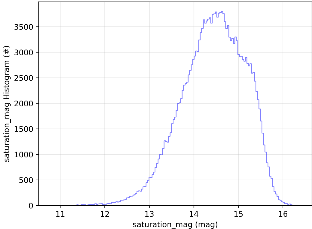
too_elab_r256_d2_griz_v3.4_10yrs All sky g band: saturation_mag Histogram
