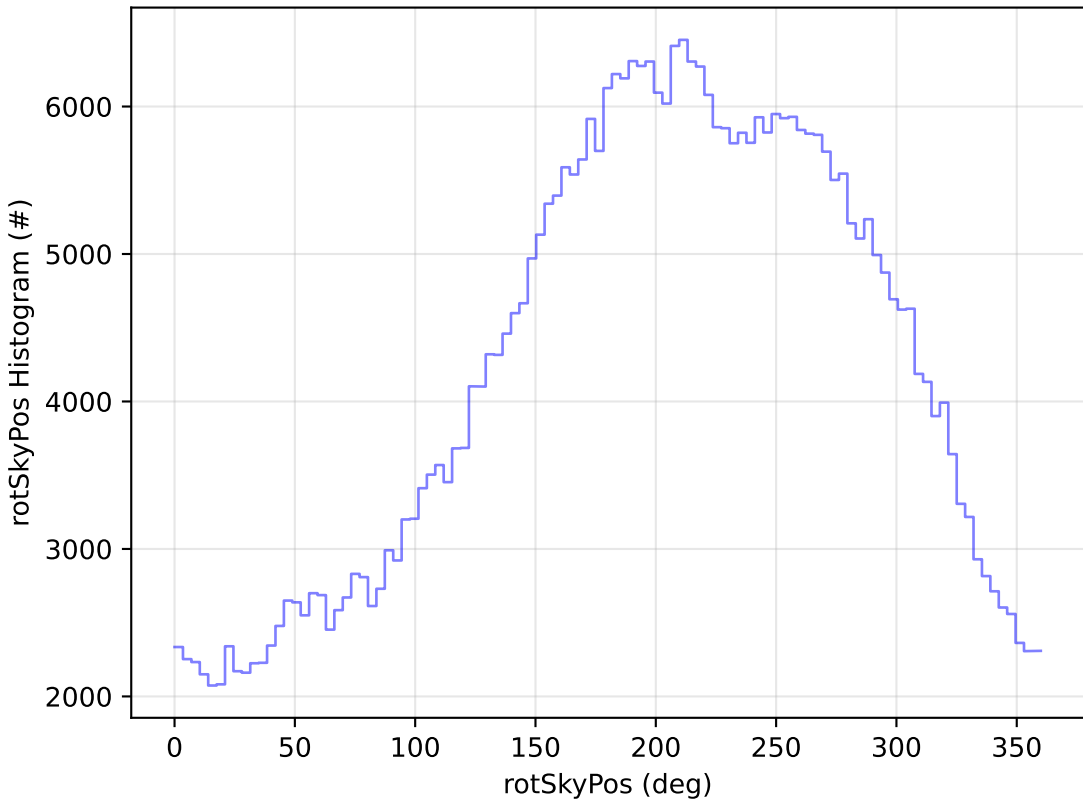
too_elab_r256_d2_griz_v3.4_10yrs WFD z band: rotSkyPos Histogram
