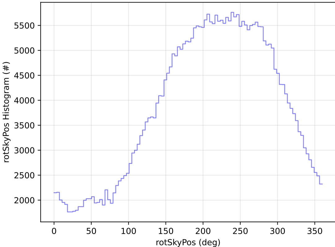
too_elab_r256_d2_griz_v3.4_10yrs WFD y band: rotSkyPos Histogram
