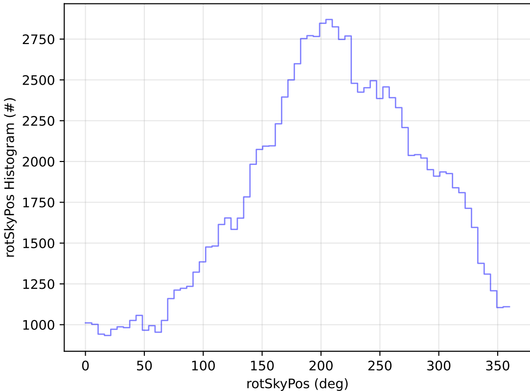
too_elab_r256_d2_griz_v3.4_10yrs WFD u band: rotSkyPos Histogram
