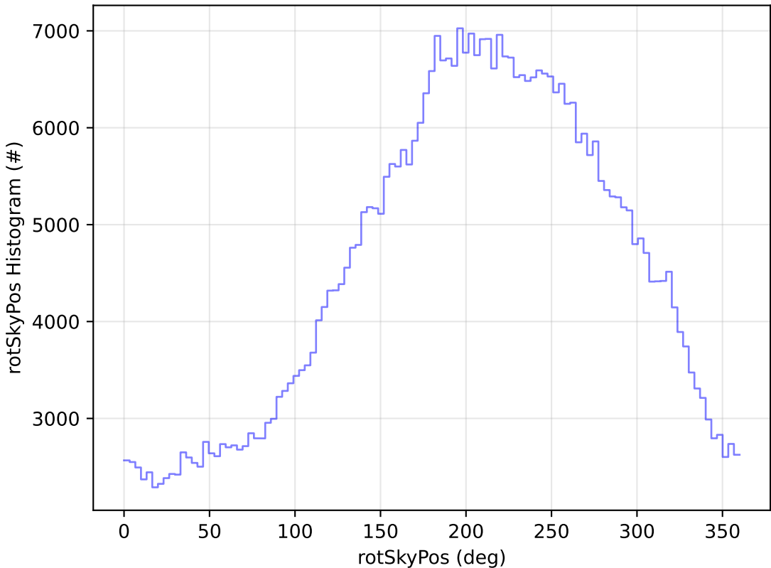
too_elab_r256_d2_griz_v3.4_10yrs WFD i band: rotSkyPos Histogram
