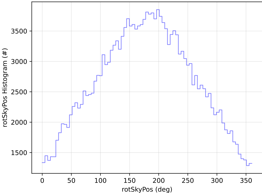
too_elab_r256_d2_griz_v3.4_10yrs WFD g band: rotSkyPos Histogram
