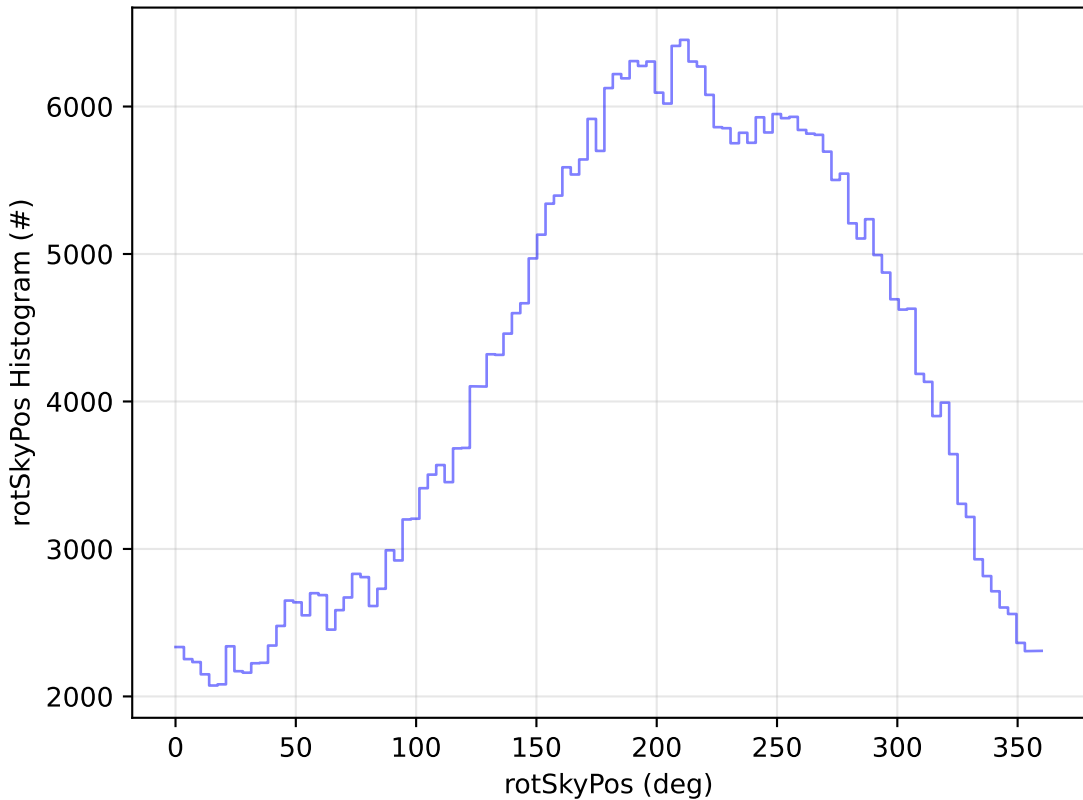
too_elab_r256_d2_griz_v3.4_10yrs All sky z band: rotSkyPos Histogram
