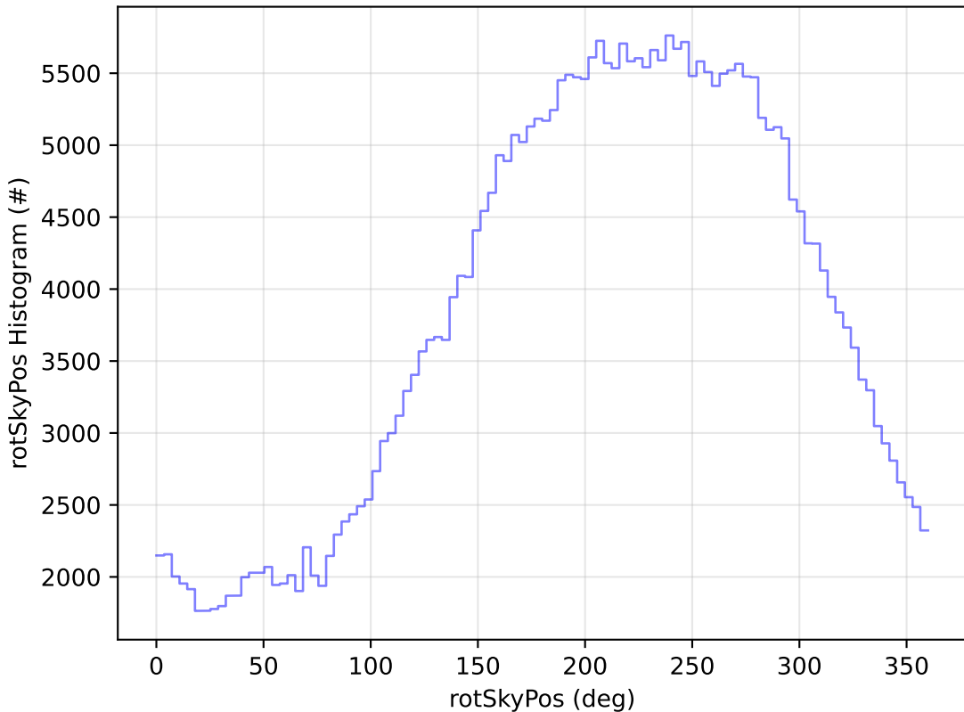
too_elab_r256_d2_griz_v3.4_10yrs All sky y band: rotSkyPos Histogram
