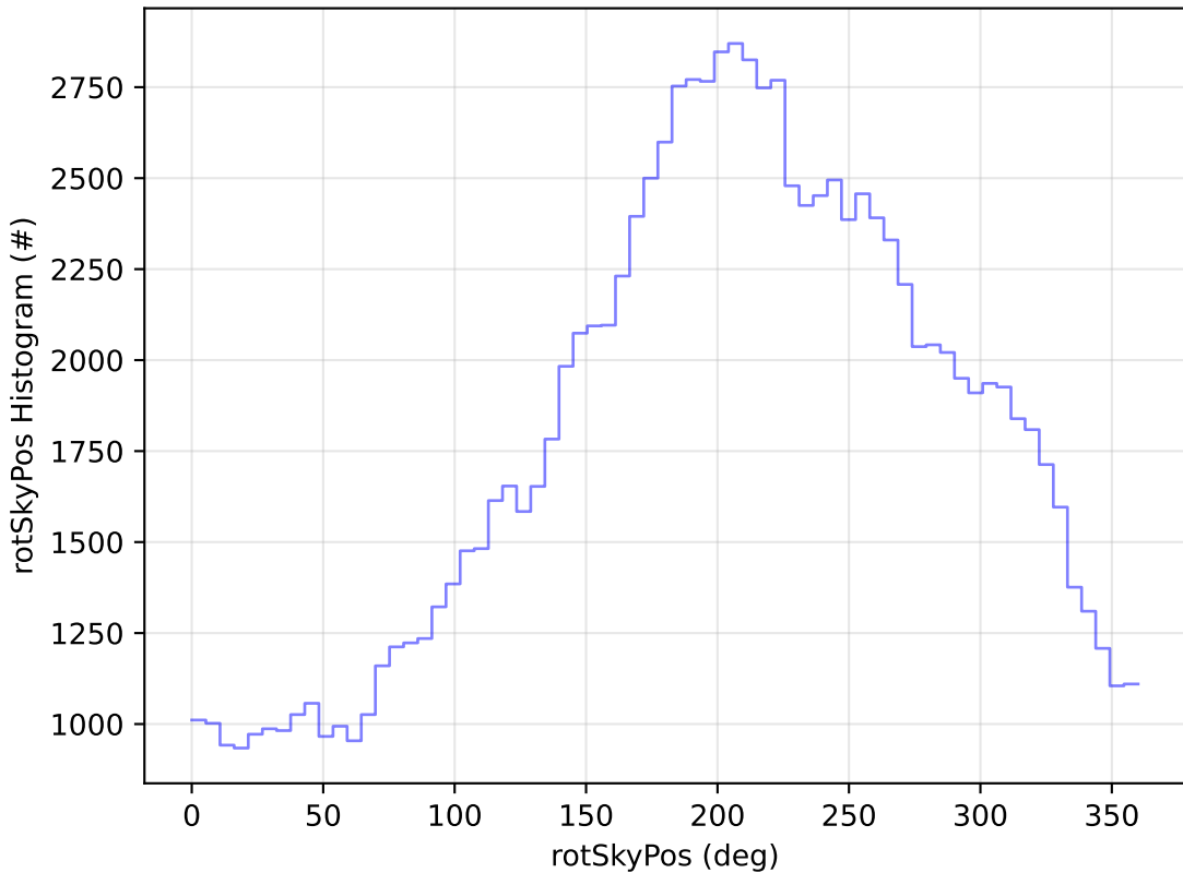
too_elab_r256_d2_griz_v3.4_10yrs All sky u band: rotSkyPos Histogram
