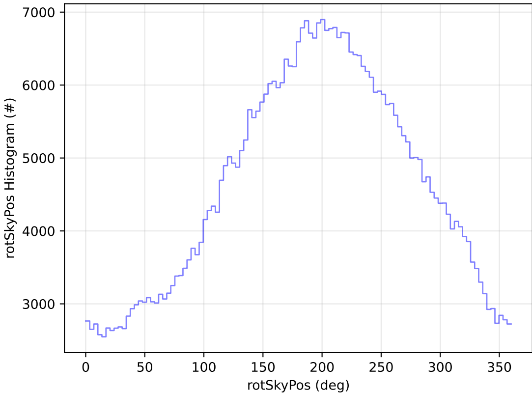
too_elab_r256_d2_griz_v3.4_10yrs All sky r band: rotSkyPos Histogram
