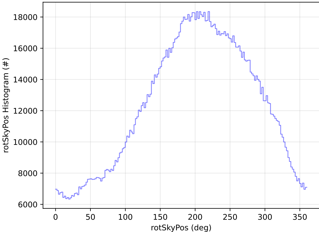
too_elab_r256_d2_griz_v3.4_10yrs All sky all bands: rotSkyPos Histogram
