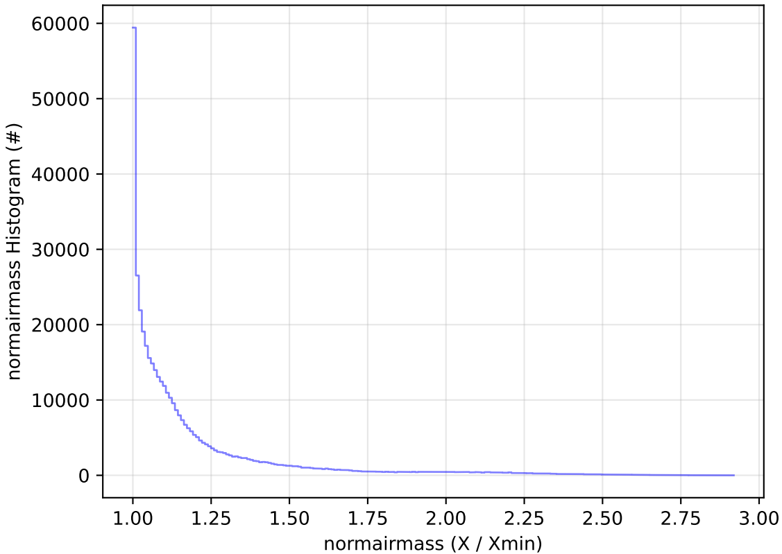
too_elab_r256_d2_griz_v3.4_10yrs WFD z band: normairmass Histogram
