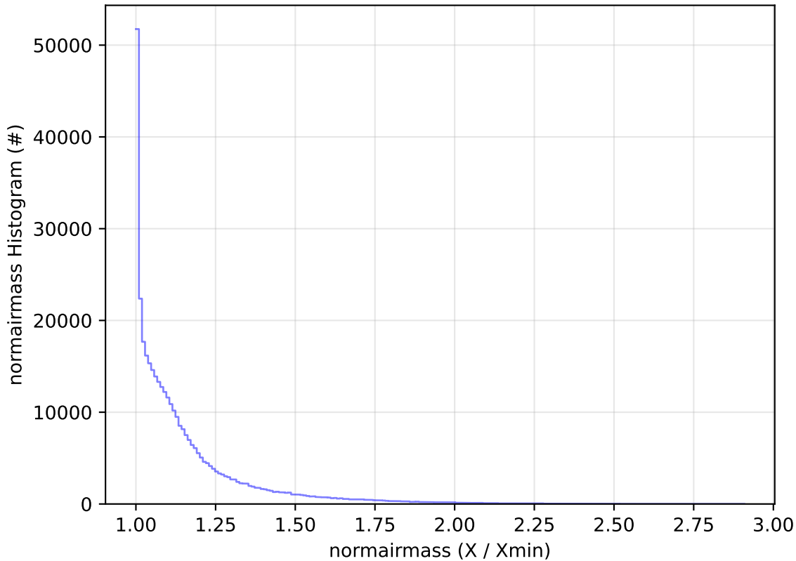
too_elab_r256_d2_griz_v3.4_10yrs WFD y band: normairmass Histogram
