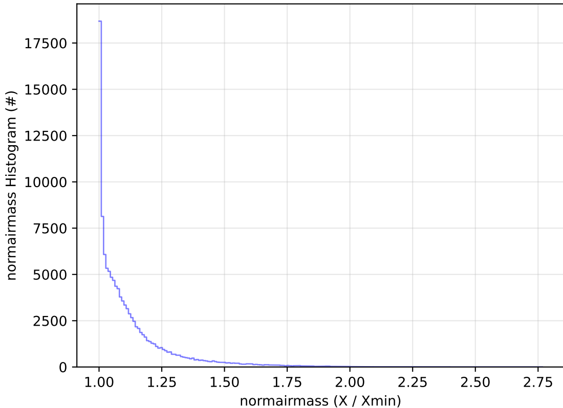
too_elab_r256_d2_griz_v3.4_10yrs WFD u band: normairmass Histogram
