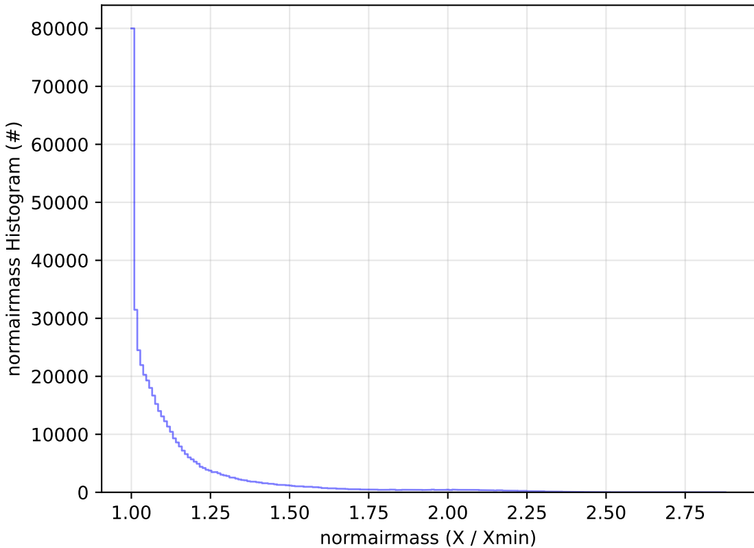
too_elab_r256_d2_griz_v3.4_10yrs WFD r band: normairmass Histogram
