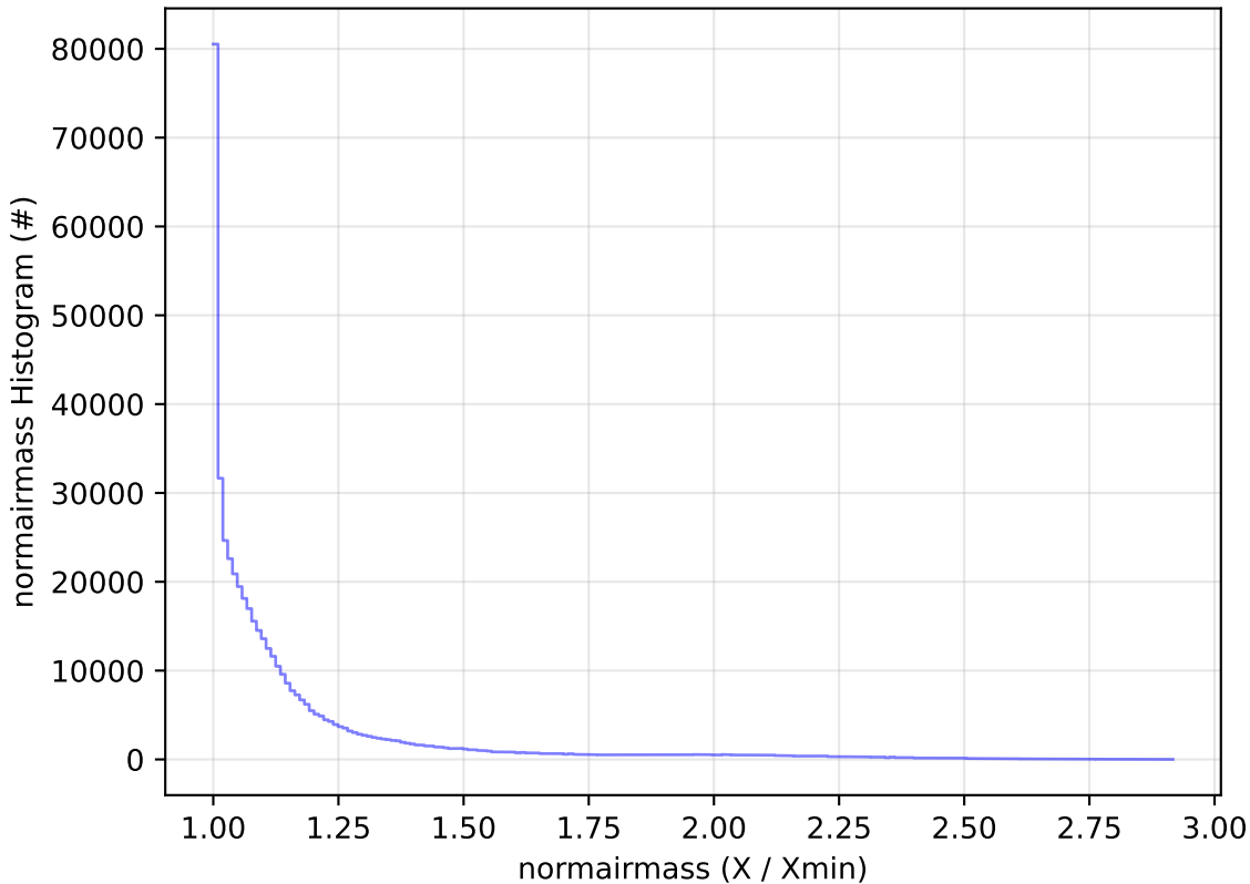
too_elab_r256_d2_griz_v3.4_10yrs WFD i band: normairmass Histogram
