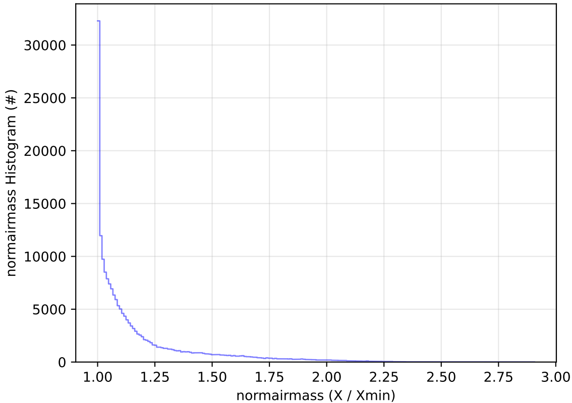
too_elab_r256_d2_griz_v3.4_10yrs WFD g band: normairmass Histogram
