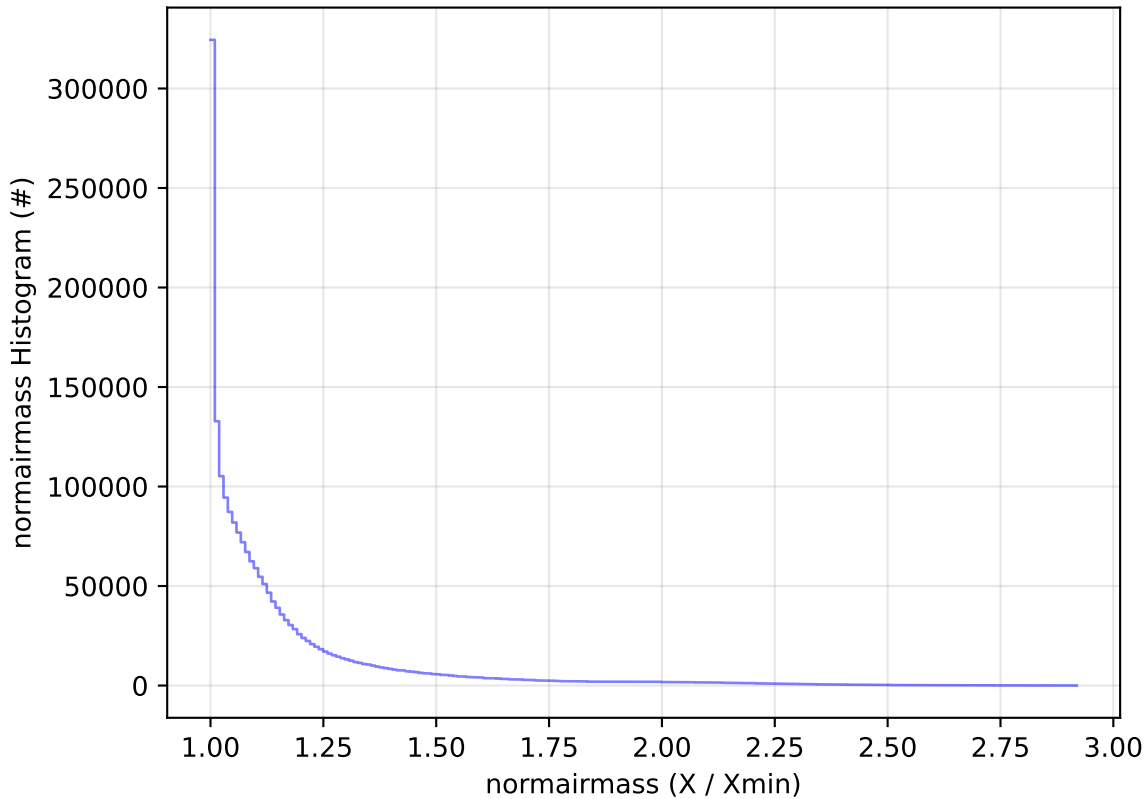
too_elab_r256_d2_griz_v3.4_10yrs WFD all bands: normairmass Histogram
