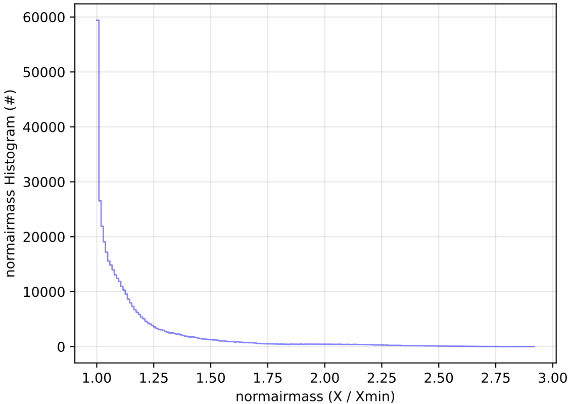
too_elab_r256_d2_griz_v3.4_10yrs All sky z band: normairmass Histogram
