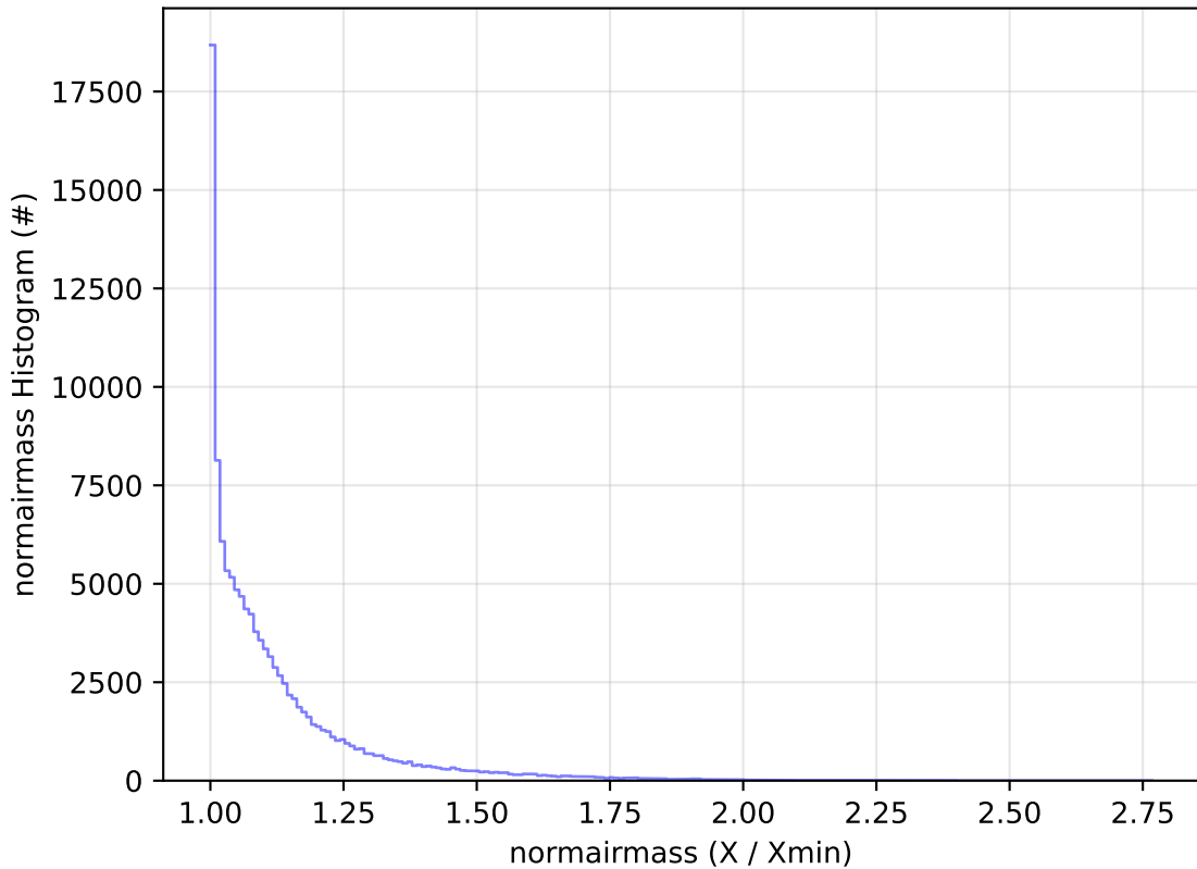
too_elab_r256_d2_griz_v3.4_10yrs All sky u band: normairmass Histogram
