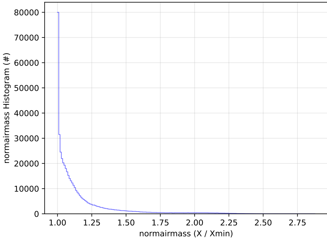
too_elab_r256_d2_griz_v3.4_10yrs All sky r band: normairmass Histogram
