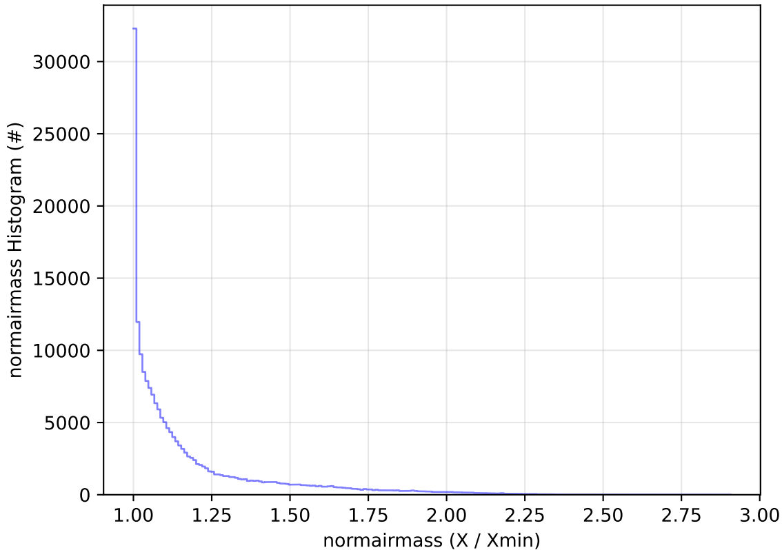
too_elab_r256_d2_griz_v3.4_10yrs All sky g band: normairmass Histogram
