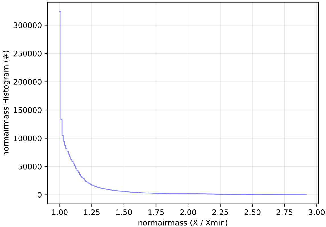
too_elab_r256_d2_griz_v3.4_10yrs All sky all bands: normairmass Histogram
