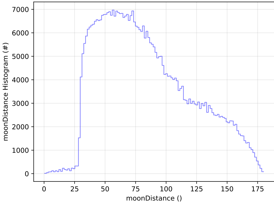
too_elab_r256_d2_griz_v3.4_10yrs WFD z band: moonDistance Histogram
