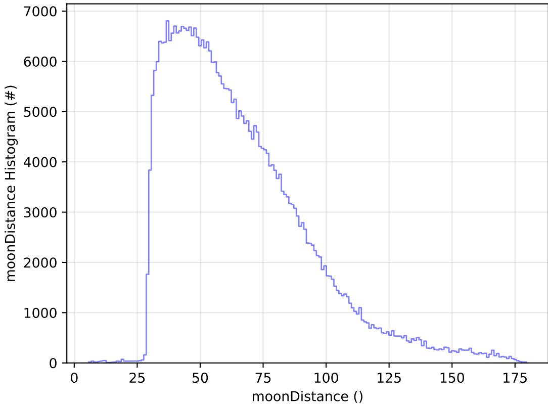
too_elab_r256_d2_griz_v3.4_10yrs WFD y band: moonDistance Histogram
