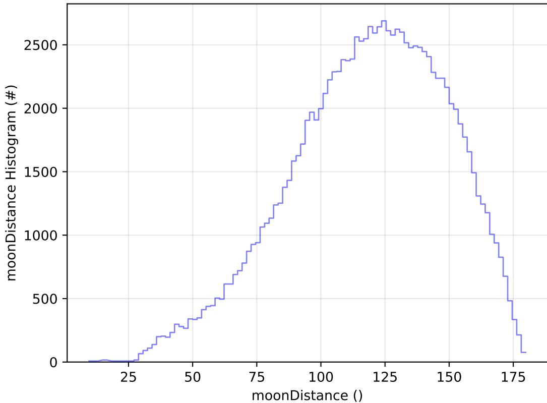
too_elab_r256_d2_griz_v3.4_10yrs WFD u band: moonDistance Histogram
