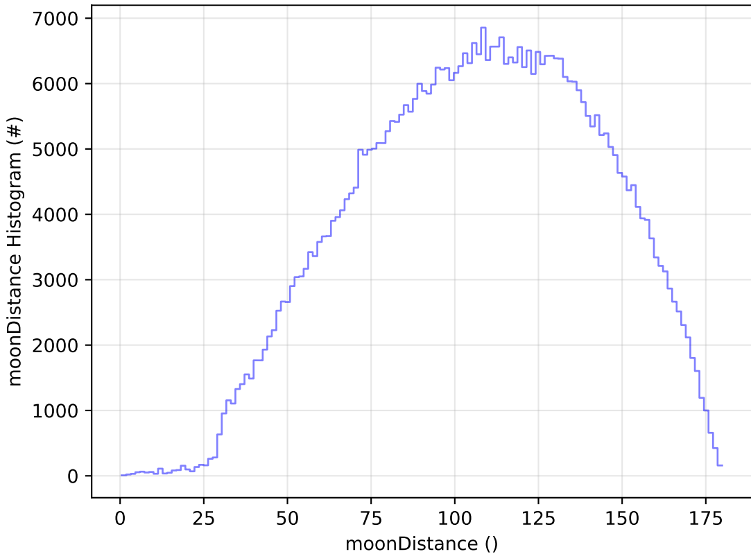
too_elab_r256_d2_griz_v3.4_10yrs WFD r band: moonDistance Histogram
