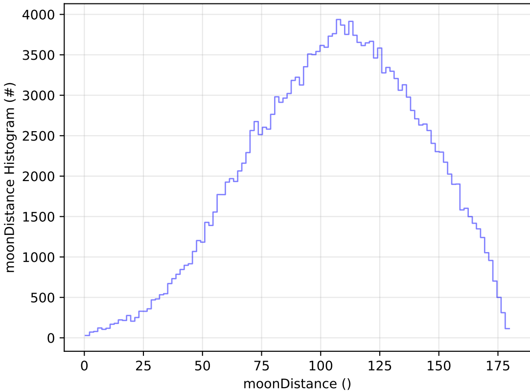
too_elab_r256_d2_griz_v3.4_10yrs WFD g band: moonDistance Histogram
