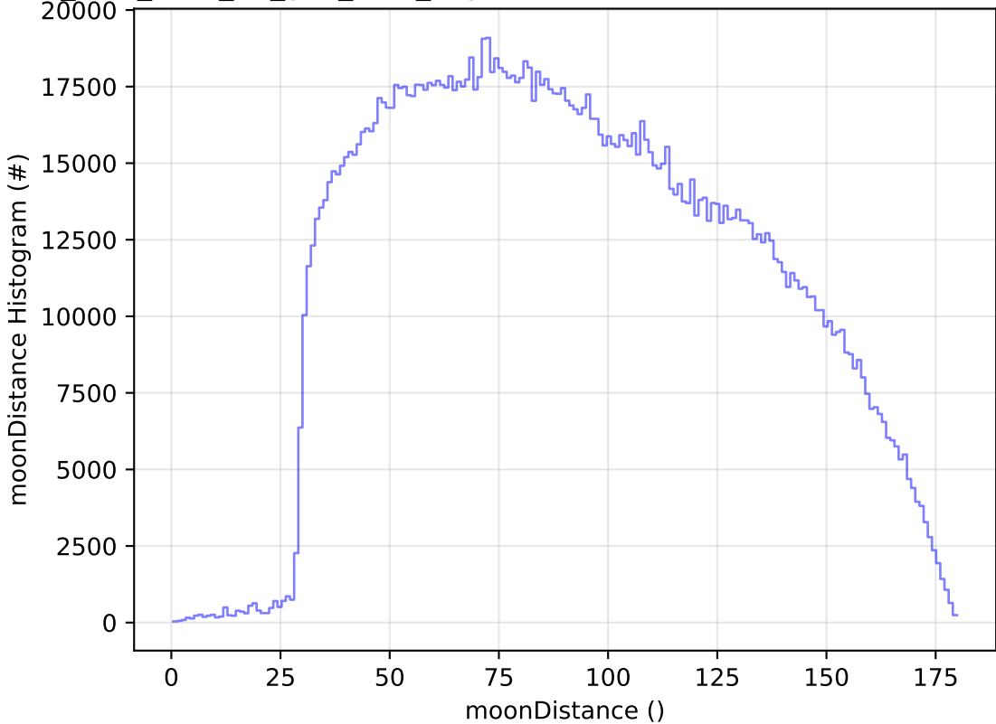
too_elab_r256_d2_griz_v3.4_10yrs WFD all bands: moonDistance Histogram
