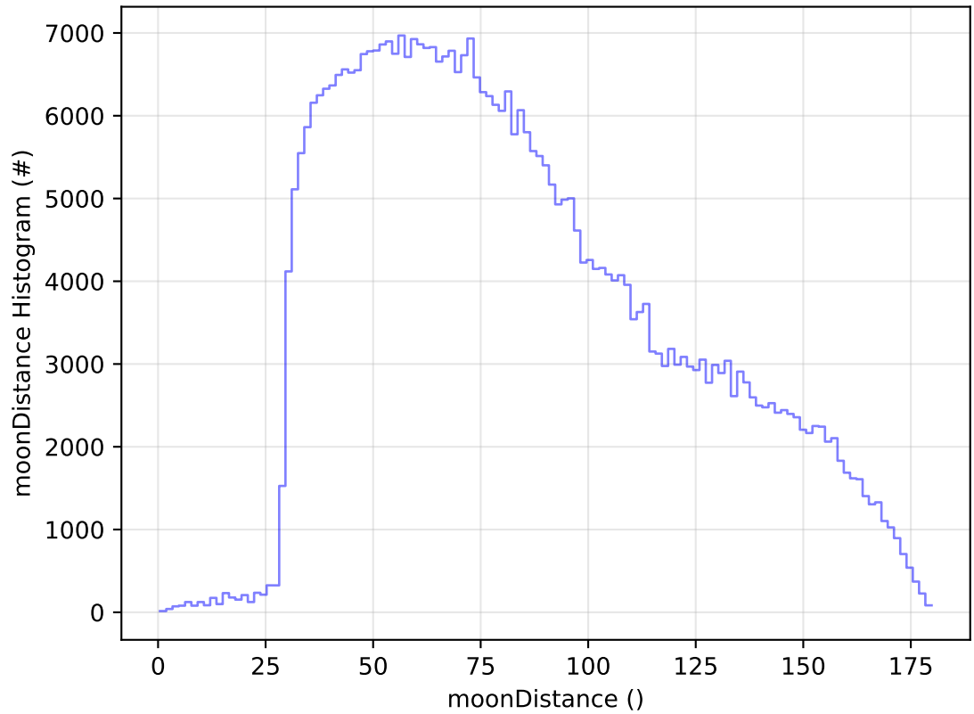
too_elab_r256_d2_griz_v3.4_10yrs All sky z band: moonDistance Histogram
