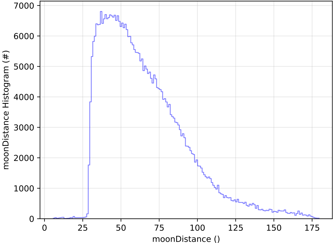
too_elab_r256_d2_griz_v3.4_10yrs All sky y band: moonDistance Histogram
