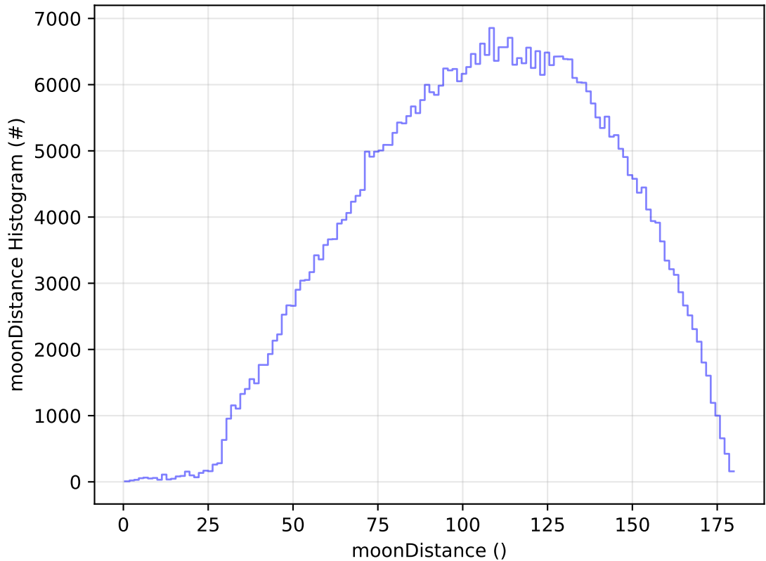
too_elab_r256_d2_griz_v3.4_10yrs All sky r band: moonDistance Histogram
