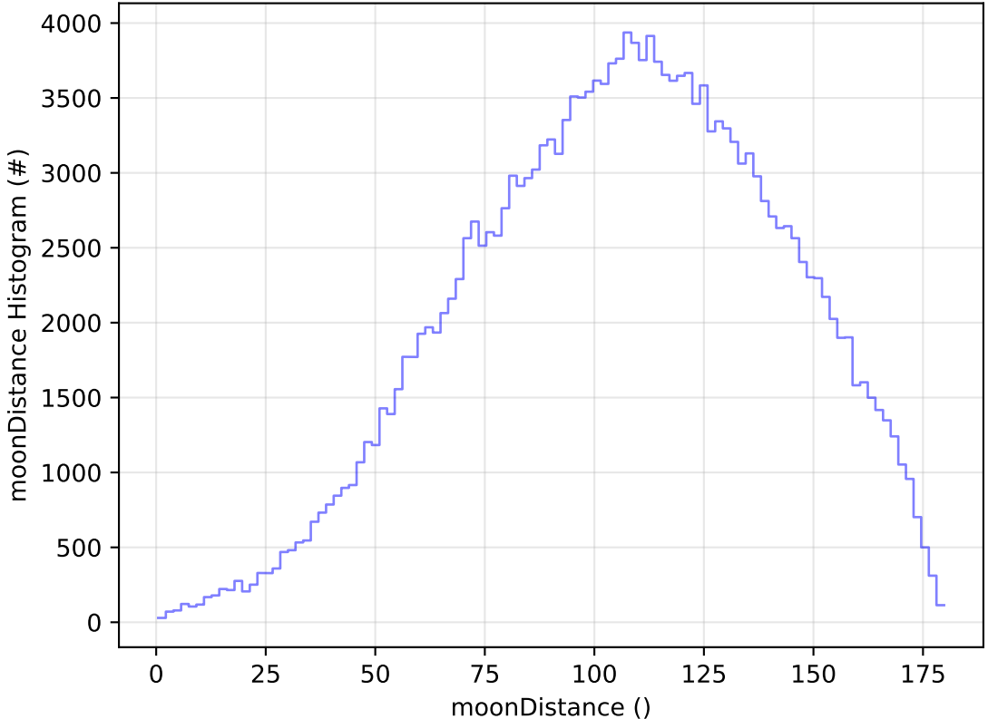
too_elab_r256_d2_griz_v3.4_10yrs All sky g band: moonDistance Histogram
