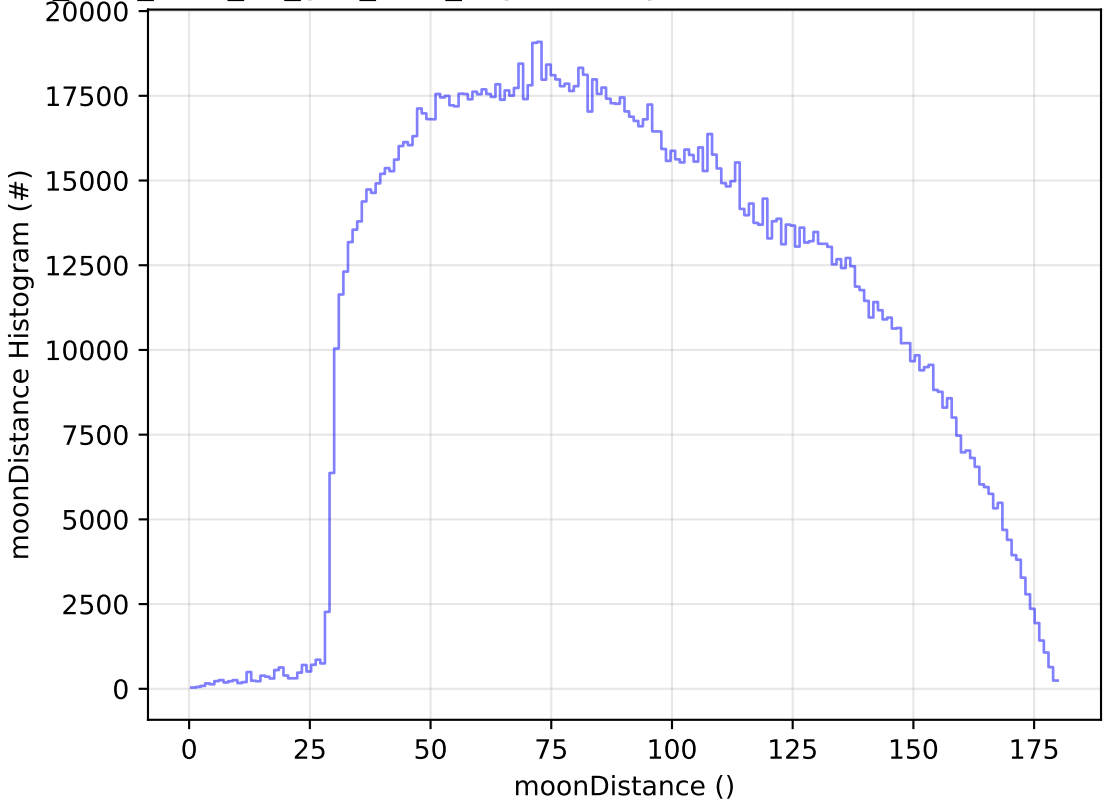
too_elab_r256_d2_griz_v3.4_10yrs All sky all bands: moonDistance Histogram
