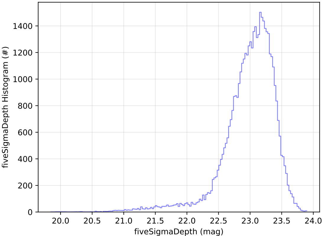
too_elab_r256_d2_griz_v3.4_10yrs Yr 1 z band: fiveSigmaDepth Histogram
