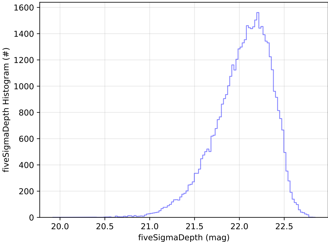
too_elab_r256_d2_griz_v3.4_10yrs Yr 1 y band: fiveSigmaDepth Histogram
