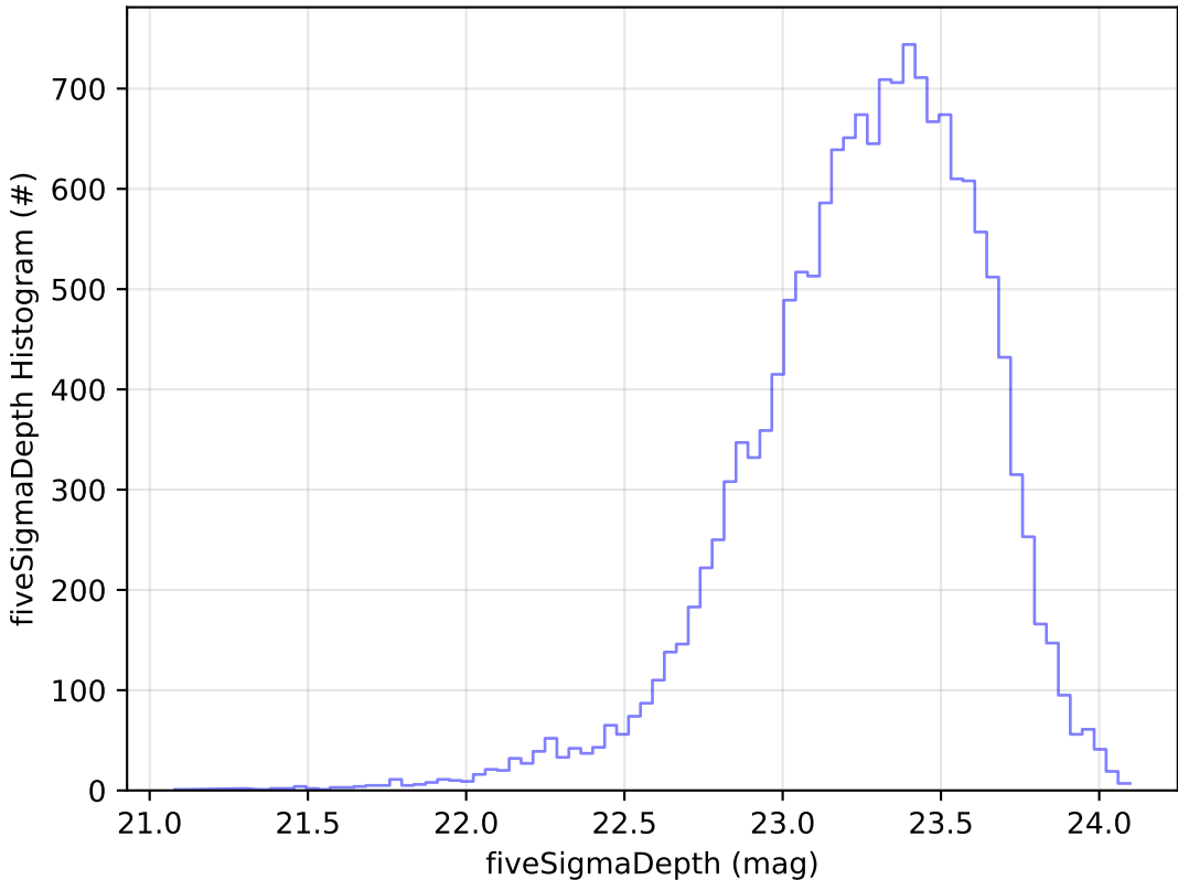
too_elab_r256_d2_griz_v3.4_10yrs Yr 1 u band: fiveSigmaDepth Histogram
